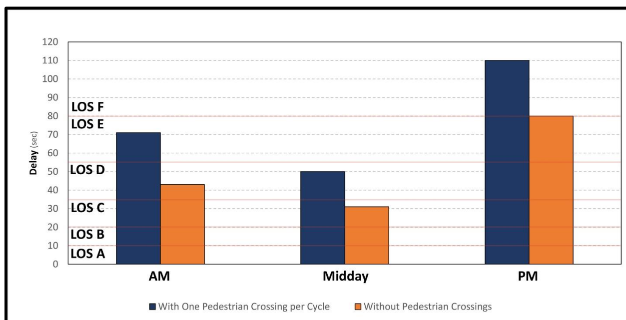
Figure 38. Comparison of Signalized Intersection Delay with or without Pedestrian Crossings of Egan Drive (Two Southbound and Three Northbound Through Lanes), Alternative Concept C2, 2040
