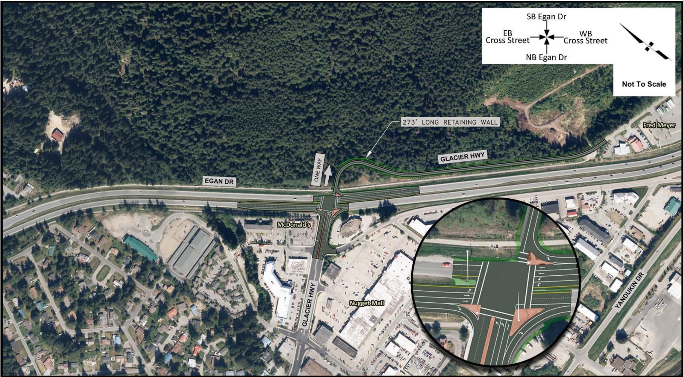
Figure 35. Concept Map, Alternative Concept C1, One-Way Extension of Glacier Highway/Lemon Spur to Glacier Highway/Nugget
