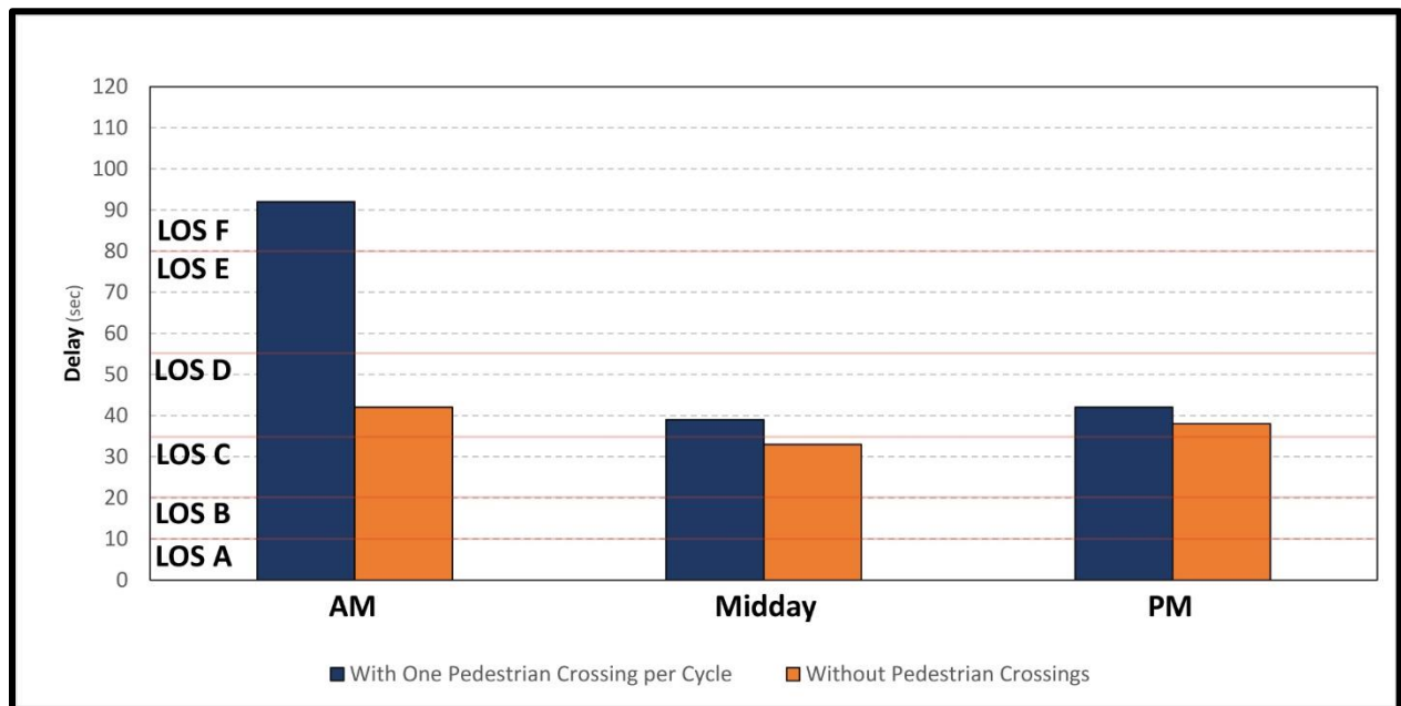
Figure 33. Comparison of Signalize Intersection Delay with or without Pedestrian Crossings of Egan Drive (Two Southbound and Three Northbound Through Lanes), Alternative Concept B, 2040
